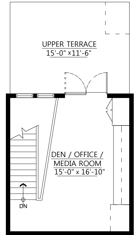
Third Floor Plan Floor Area: 285 sq.ft.
