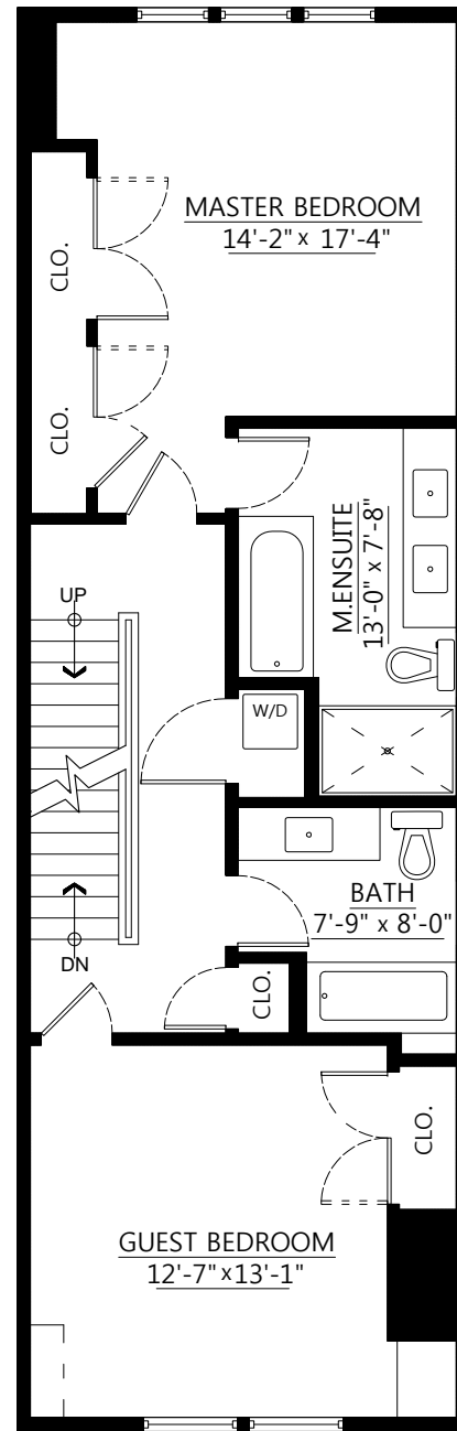
Second Floor Plan Floor Area: 802 sq.ft.
